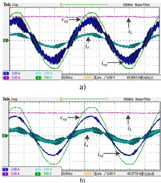
Fig. 9. PM machine, three-phase charging mode: a) is without interleaving, (b) is with interleaving. Traces as in Fig. 8.
