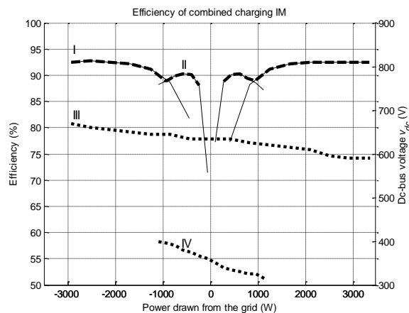
Fig. 19. Induction machine, combined single-phase and three-phase charging: efficiency without interleaving (I – three-phase grid, II – single phase grid) and applied dc-bus voltage (III – three-phase grid, IV – single phase grid). Suggested combination of single-phase and three-phase connection for best efficiency performance indicated with bold dashed segments of lines I and II.
