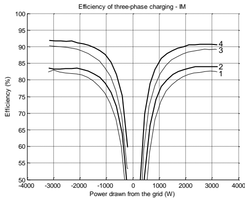
Fig. 13. Induction machine, three-phase charging mode, efficiency: traces 1, 3 are with interleaving, while 2, 4 are without interleaving; traces 1, 2 are with the dc/dc converter, while 3, 4 are without dc/dc converter.
