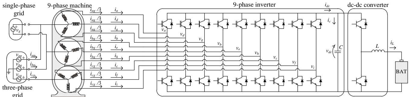
Fig. 1. Topology of the nine-phase fast integrated on-board battery charger in three-phase charging mode.
