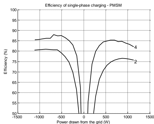
Fig. 18. PM machine, single-phase charging mode, efficiency without interleaving. Trace 4 is without dc/dc converter, trace 2 is with the dc/dc converter.
