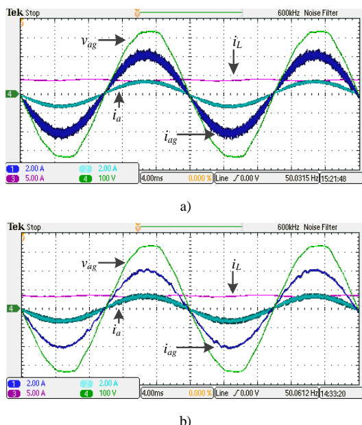
Fig. 8. PM machine, single-phase charging mode: a) without interleaving, (b) with interleaving (CH1 - grid phase current i_{ag} , CH2 - machine phase current i_a , CH3 - battery charging current i_L , CH4 - grid phase voltage v_{ag} ).
