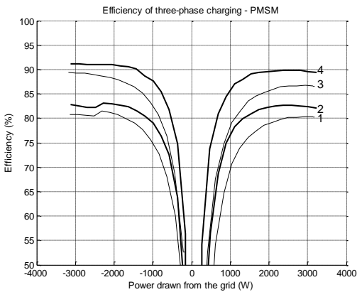
Fig. 14. PM machine, three-phase charging mode, efficiency: traces 1, 3 are with interleaving, while 2, 4 are without interleaving; traces 1, 2 are with the dc/dc converter, while 3, 4 are without dc/dc converter.
