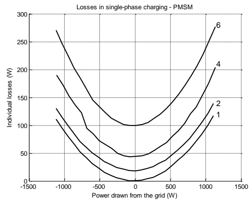
Fig. 17. PM machine, single-phase grid connection: losses in the machine (1, 2), machine plus converter (4), and total losses including the dc/dc converter (6) without interleaving.
