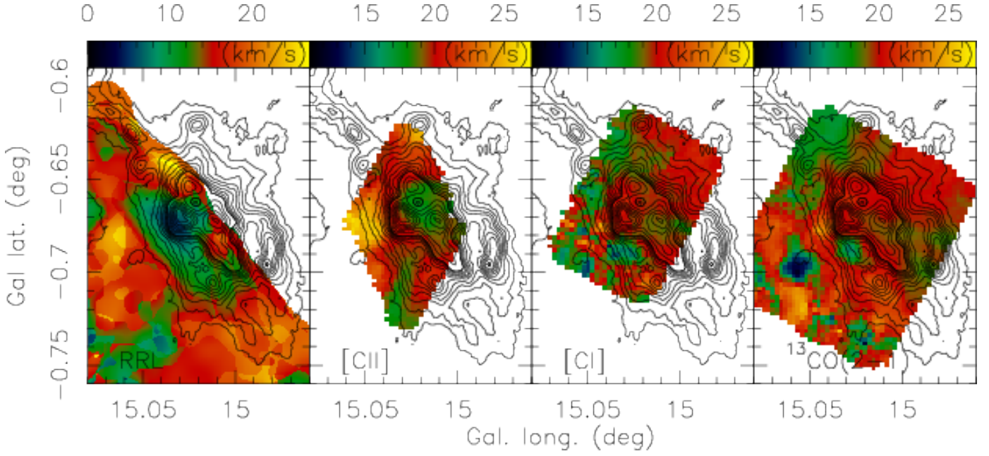
Fig. 13. Compilation of first moment maps (intensity-weighted peak velocities) toward M17 of the THOR RRL data (left panel) with ionized carbon, atomic carbon, and molecular carbon (second to fourth panel) taken from Pérez-Beaupuits et al. (2012, 2015). The color scale for the recombination lines is from 0 to 27 km s -1 , for the others from 11 to 27 km s -1 . The contours show the 870 μm continuum data from the ATLASGAL survey starting at a 4σ level of 200 mJy beam -1 .
