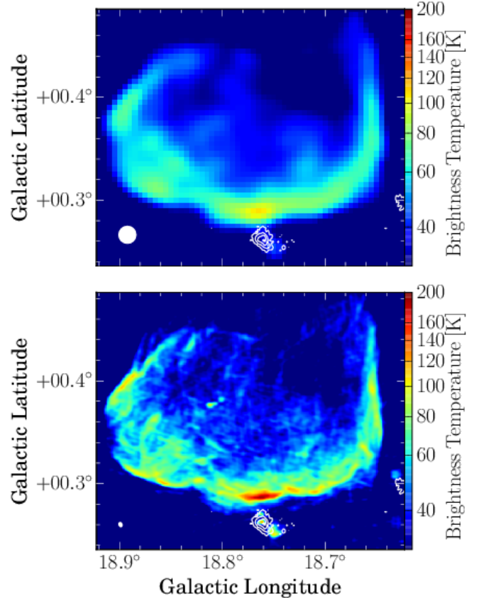
Fig. 6. The two panels present the 1.4 GHz continuum emission toward the supernova remnant G18.8+0.3. While the top panel shows the old VGPS data, the bottom panel presents the vast improvement obtained with our new THOR+VGPS data. The contours in both panels present the 870 \mu\text{m} continuum data from the ATLASGAL survey (Schuller et al., 2009).
