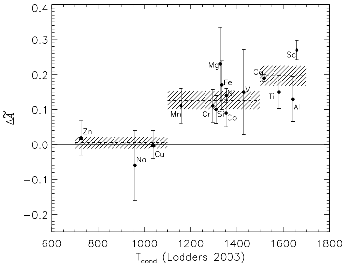
Fig. 1. Differential abundances of #52 and #45 as a function of the condensation temperature. The plotted \Delta\tilde{A} values are those reported in Table 1. The triangles are from Table 2. The condensation temperatures are taken from Lodders (2003). The horizontal dashed lines represent the weighted means of the differential abundances within each class of elements (i.e., volatiles, and moderately and super refractory elements). The bands represent the weighted standard deviation of the mean.
