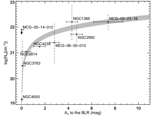
Figure 4. A_V to the broad line region versus X-ray absorbing column N_H , adapted from a similar figure by Bartscher et al. (2016). The vertical dashed lines denote the range of absorbing columns in the literature, which indicates the minimum variability for each object. The N_H value for MCG-05-14-012 is an upper limit. The thick grey line represents the Galactic standard gas-to-dust ratio (Predehl & Schmitt 1995; Nowak et al. 2012).
