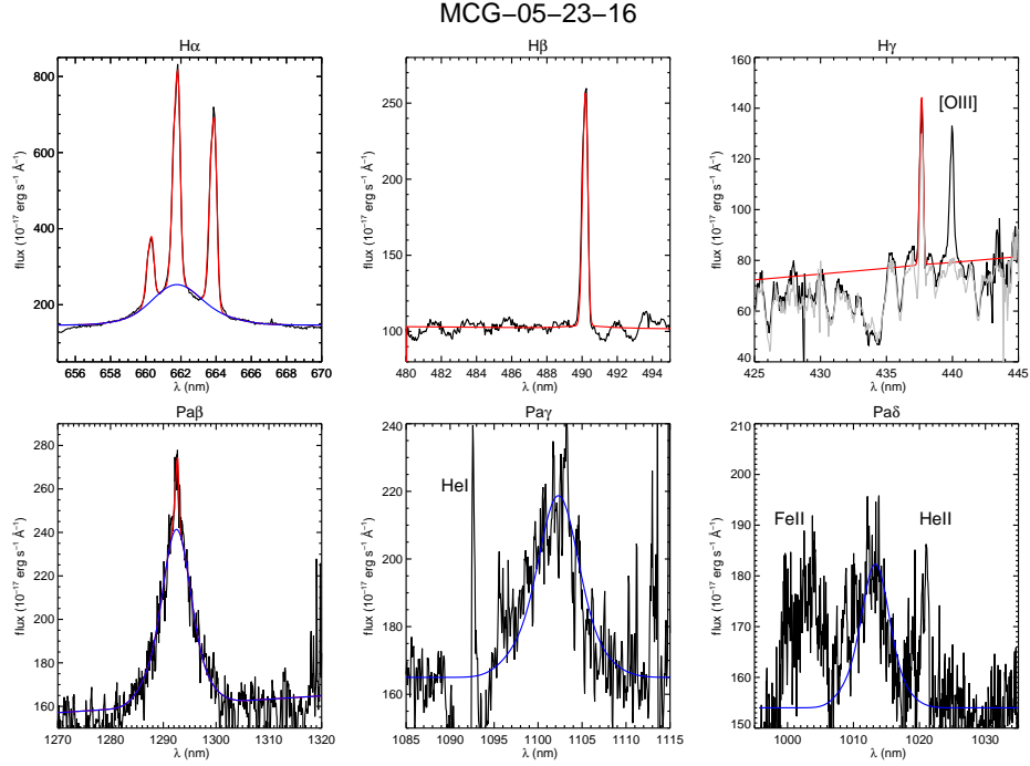
Figure 6. Observed H \alpha , H \beta , H \gamma , Pa \beta , Pa \gamma and Pa \delta line profiles from an integrated spectrum of the inner l'2 (black), fitted broad (blue) and broad plus narrow (red) profiles lines. On the H \gamma panel, we show in grey a combination of the fitted H \gamma profile and the spectrum of an inactive galaxy, in order to illustrate that most of the differences between the observed and fitted profiles are due to the shape of the underlying stellar continuum. On the Pa \gamma panel, broad HeI was subtracted from the spectrum.
