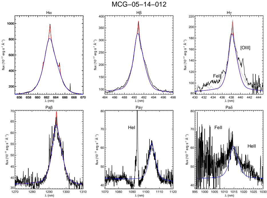
Figure 7. Observed H \alpha , H \beta , H \gamma , Pa \beta , Pa \gamma and Pa \delta line profiles from an integrated spectrum of the inner l'2 (black), fitted broad (blue) and broad plus narrow (red) profiles lines. On the H \gamma panel, we show in grey a combination of the fitted H \gamma profile and the spectrum of an inactive galaxy, in order to illustrate that most of the differences between the observed and fitted profiles are due to the shape of the underlying stellar continuum. Excess emission on the wings of the broad H \gamma line are due to [OIII] and FeII multiplets. On the Pa \gamma panel, broad HeI was subtracted from the spectrum.
