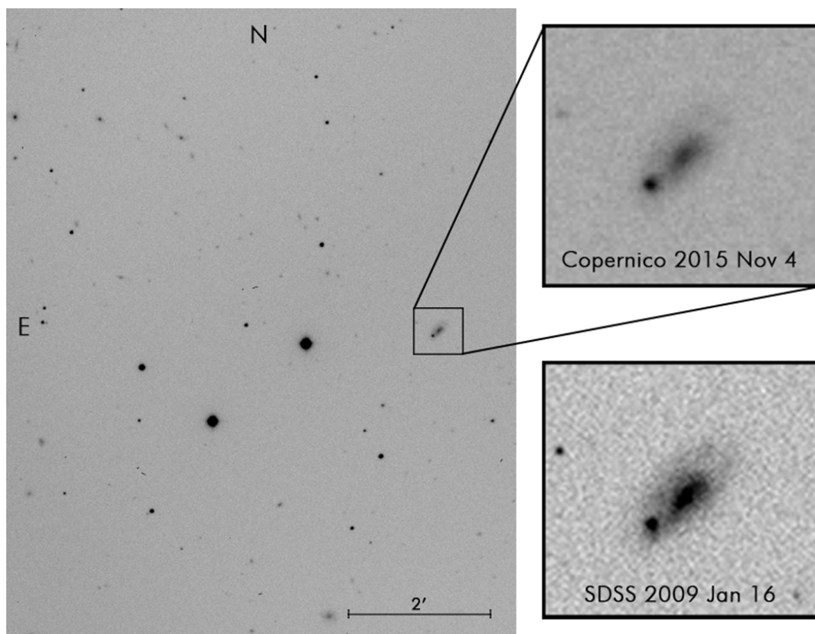
Figure 1. Images of the field of iPTF15dld in r -band (exposure time of 120 seconds) taken on 4 November 2015 with the 1.82m Copernico telescope (larger panel on the left and enlargement centered on the host galaxy on the top-right smaller panel) and from the SDSS prior to explosion (smaller bottom-right panel, covering the same area as the small top-right panel).
