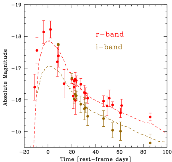
Figure 3. Light curves of iPTF15dld in r -band (red circles) and i -band (brown circles), corrected for Galactic extinction ( A_V = 0.085 ). At z = 0.047 , the central wavelengths of these bands correspond to 5980 Å and 7328 Å, respectively. The time origin corresponds to the maximum of the r -band light curve. For comparison, we overlaid the light curves of the type Ic SN 2007gr at identical reference wavelengths (dashed curves; see text for the construction of these templates). The “ r -band”-equivalent template of SN 2007gr was brightened by 0.7 magnitudes for best match with iPTF15dld.
