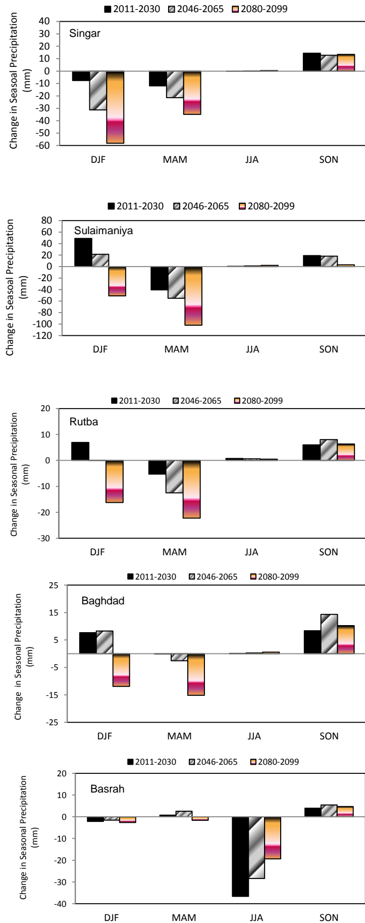
Fig 7 The differences of precipitation between the future periods and the baseline period in the studied sites
