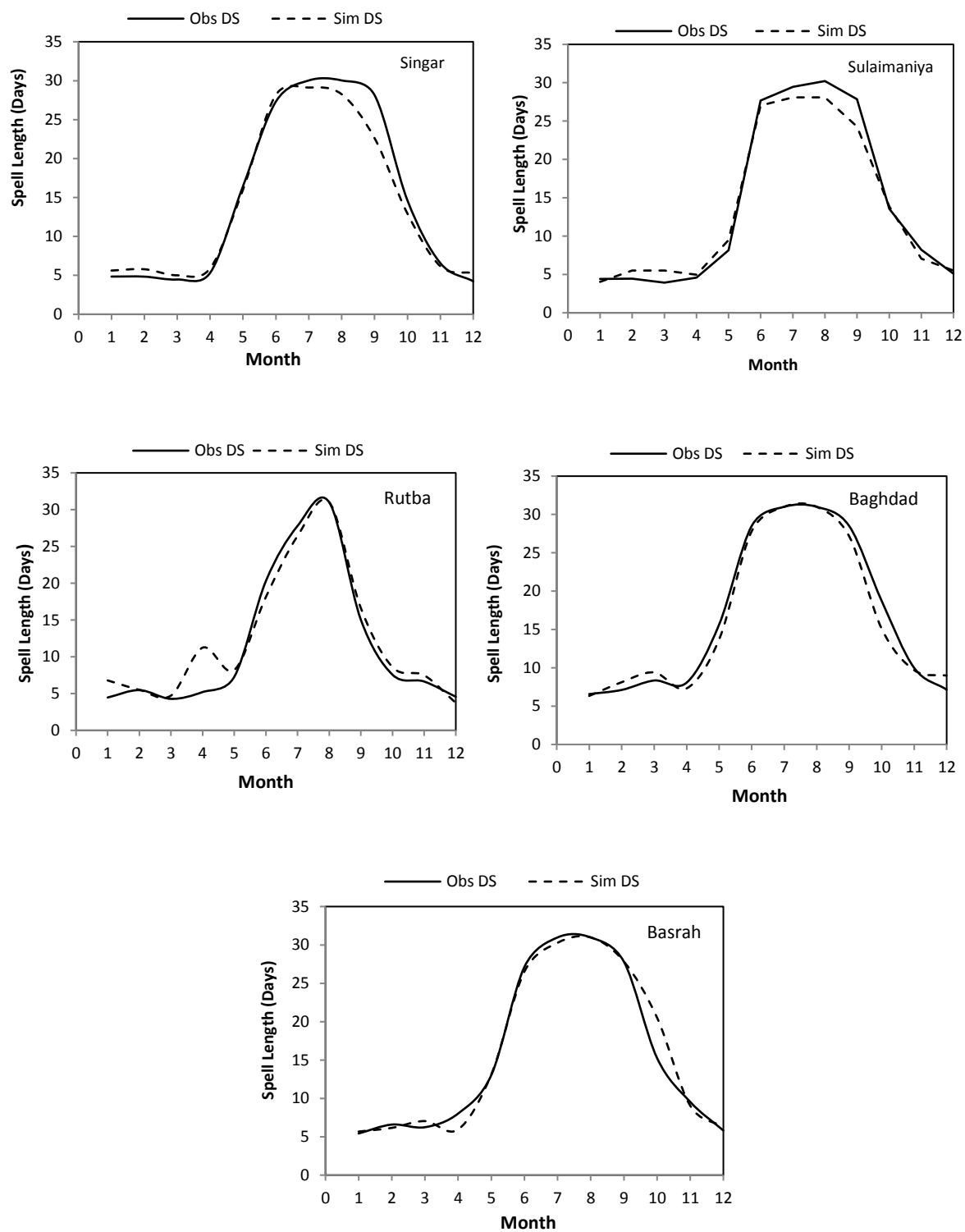
Fig 4 Comparison of observed and simulated averag dry spell lengths at studied sites
