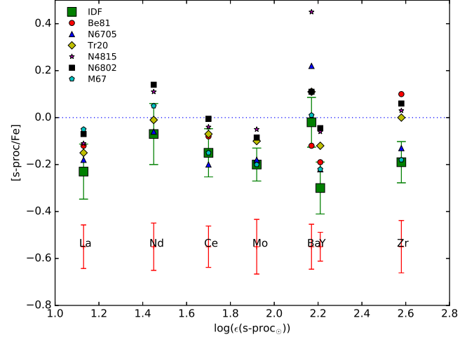
Fig. 10. Cluster median [s\text{-proc}/Fe] as a function of \log(\epsilon(s\text{-proc}_{\odot})) , where \log(\epsilon(s\text{-proc}_{\odot})) is the G07 solar abundance. The s -process element names and the median of the s -process abundance standard deviations of five GES IOCs are indicated in the bottom of the panel. The median abundances and standard deviations of the inner disk field (IDF) giants are labeled as green squares with error bars. The symbols of the five GES IOCs and M 67 are indicated in the top left. The dotted line represents [s\text{-proc}/Fe] = 0 .
