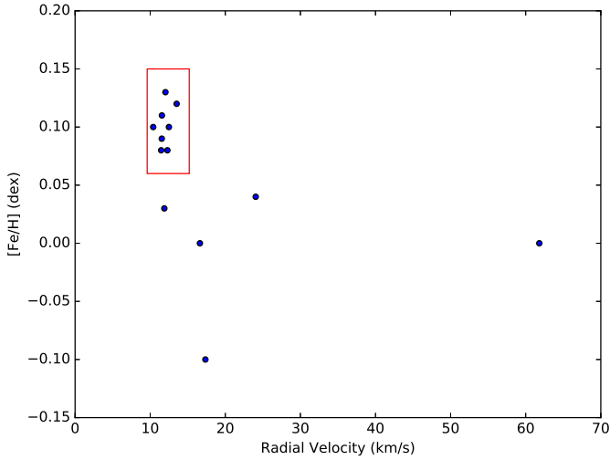
Fig. 1. [\text{Fe}/\text{H}] as a function of radial velocity (RV). All stars observed with UVES (Ultraviolet and Visual Echelle Spectrograph) are plotted. Selected cluster members are those inside the rectangle. The rectangle indicates the region that satisfies 9.6 < \text{RV} < 15.2 \text{ km s}^{-1} and 0.06 < [\text{Fe}/\text{H}] < 0.15 \text{ dex} .
