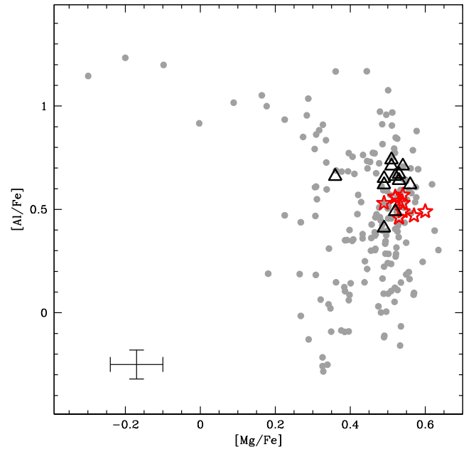
Figure 2. [Al/Fe] abundance ratio as a function of [Mg/Fe] for the 11 UVES targets of NGC 6362 analysed in this work (red stars), for 12 giants belonging to M 4 (black triangles), and for 17 Galactic GCs (grey dots, data from Carretta et al. 2009). Typical errors are shown in the bottom left-hand region of the plot.
