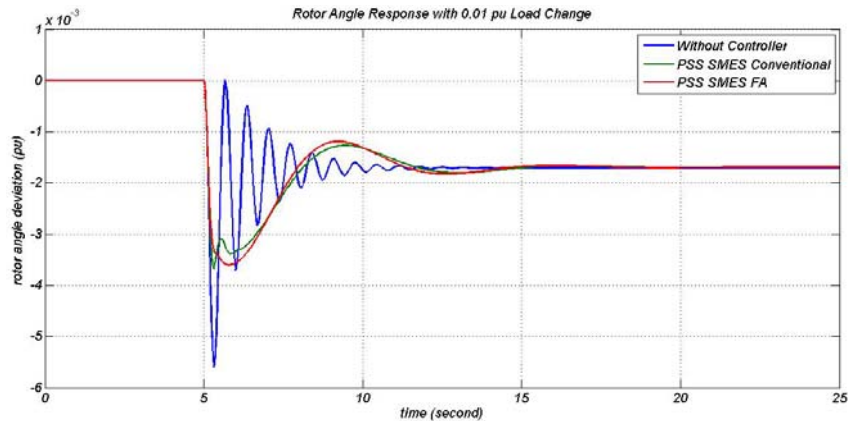
Figure 10. Rotor Angle Response Comparison
