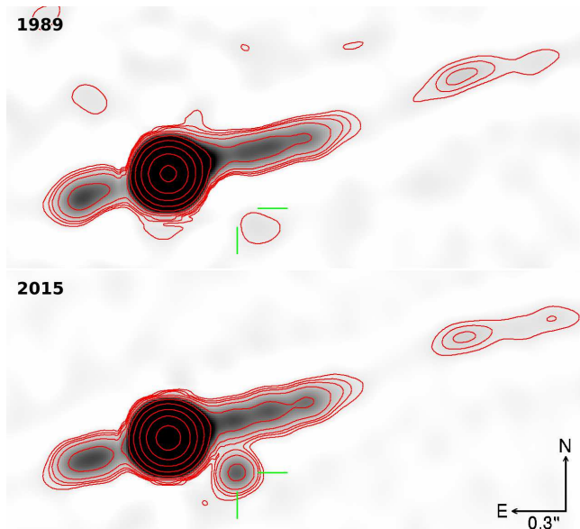
FIG. 1.— Discovery images of the off-nuclear radio transient Cygnus A-2. Both images show VLA observations at 8.5 GHz, using spacings of >150\lambda only. The scale and contours are the same for both panels (the first five contours are 0.5, 0.85, 1.2, 2, and 4 mJy/beam). A point source is detected approximately 0.42'' west-southwest of the nucleus in the new observations (location designated by the green crosshairs). No source at this location was present in 1989.
