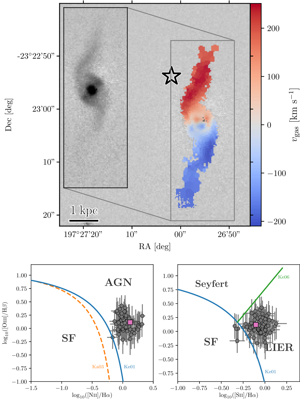
Figure 4. Top: velocity map of ionized gas in NGC 4993. Velocities are the offsets of [N II] \lambda 6583 emission. The location of the transient is indicated with a star symbol. Inset shows an [N II] \lambda 6583 narrowband image constructed from the MUSE data cube. The motion of the “arm”-like features is in the radial velocity plane, implying they are edge-on. Bottom: emission line ratios in NGC 4993. Each point represents a spaxel bin where all the diagnostic lines are detected as a signal-to-noise ratio of >2 . Dividing lines of Kauffmann et al. (2003; pure star formation, orange dashed), Kewley et al. (2001a; theoretical star formation limit, blue) and Kewley et al. (2001b; Seyfert vs. LIER, green) are shown. The ionized gas regions in NGC 4993 are inconsistent with being driven by star formation (SF) and are better described as extended LIERs (see Sarzi et al. 2010; Singh et al. 2013). The few bins formally within theoretical SF limits show velocity dispersions \sigma_{\text{gas}} > 100 \text{ km s}^{-1} , inconsistent with typical H II regions that show tens of \text{km s}^{-1} . The position of the integrated emission lines (summing all bins) is shown by a square on each plot.
