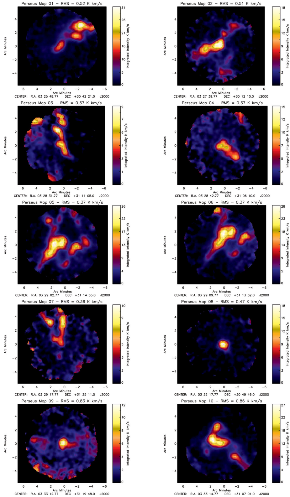
Figure 3. The Perseus and W3 integrated intensity maps.
