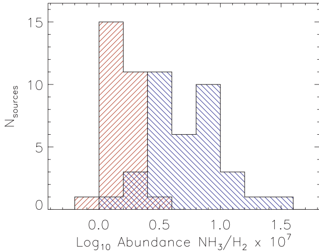
Figure 14. \text{NH}_3 fractional abundances found in Perseus (red) and W3 (blue) cores.
