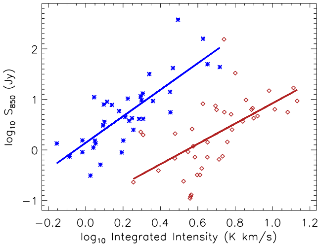
Figure 7. Log 10 integrated 850 \mu m fluxes versus NH 3 log 10 integrated intensities for source associations in Perseus (red diamonds) and W3 (blue stars).
