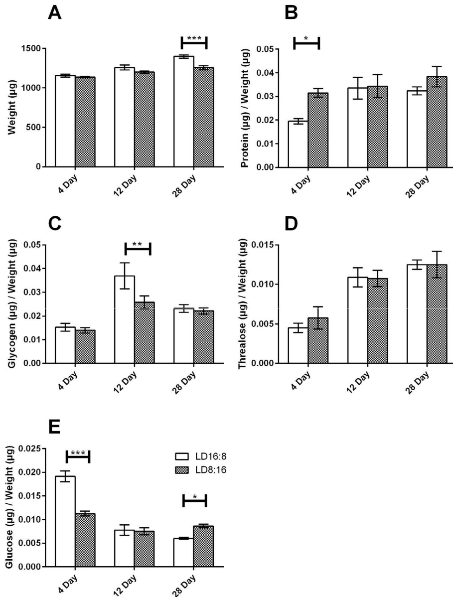
Fig. 6. Photoperiod and time effects on metabolites accumulation. Fresh weight (A) of D. melanogaster females (MREN from Rende, south Italy). Samples were collected after 4, 12 and 28 days at 12 °C either at LD8:16 or LD16:8. For the same samples, ratios protein/weight (B), glycogen/weight (C), trehalose/weight (D) and glucose/weight (E) are given. Bars represent means and SEMs. †Indicates Duncan's post hoc test p < 0.05 , ** p < 0.01 , *** p < 0.001 .
