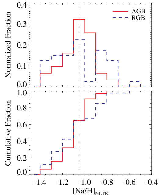
Fig. 8. Histograms of [\text{Na}/\text{H}] ( top ) and cumulative distribution functions ( bottom ) of our AGB and RGB sample in NGC 2808. The black vertical dash-dotted line separates 1P and 2P stars using Carretta et al. (2009b) criteria (see text).
