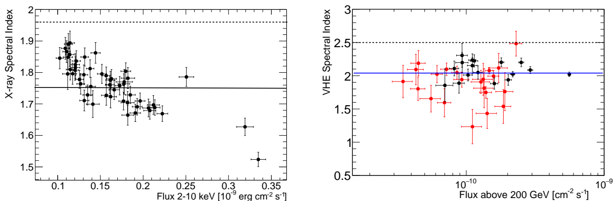
Fig. 4. Left Panel: Swift /XRT X-ray power-law spectral index vs flux in the 2-10 keV band. Right Panel: Measured VHE power-law spectral index vs VHE Flux above 0.2 TeV. Red points represent VERITAS data and black points MAGIC data. The data are EBL corrected using Franceschini et al. (2008). The Swift /XRT spectrum of Mrk 501 is often curved, and can be described at keV energies with a spectral index that is typically between 1.8 and 2.1, while the VHE spectral index measured with MAGIC and VERITAS during typical non-flaring activity is about 2.5 (Abdo et al. 2011; Aleksić et al. 2015a). The typical spectral indices at X-ray and VHE are marked with a dashed line. For comparison purposes, the panels depict with solid lines the result of a fit with a constant to the X-ray and VHE spectral indices.
