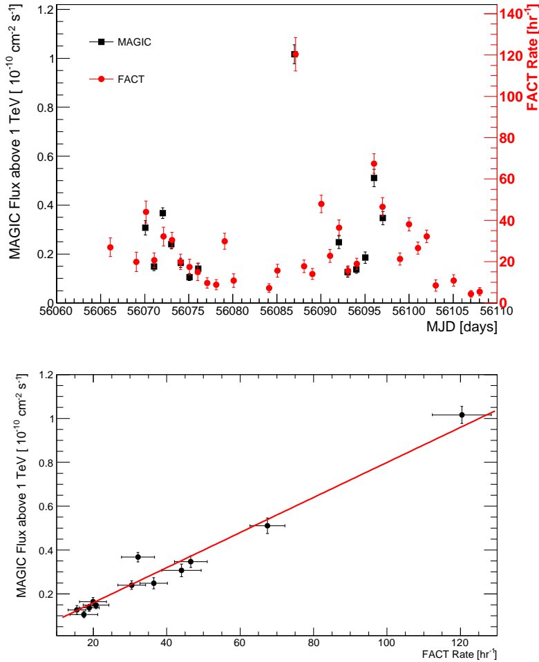
Fig. 9. Top panel: superposition of the FACT excess rates and MAGIC light curve above 1 TeV. Bottom panel: correlation between the FACT excess rate and the MAGIC flux above 1 TeV on the 12 days when data were taken by both instruments.
