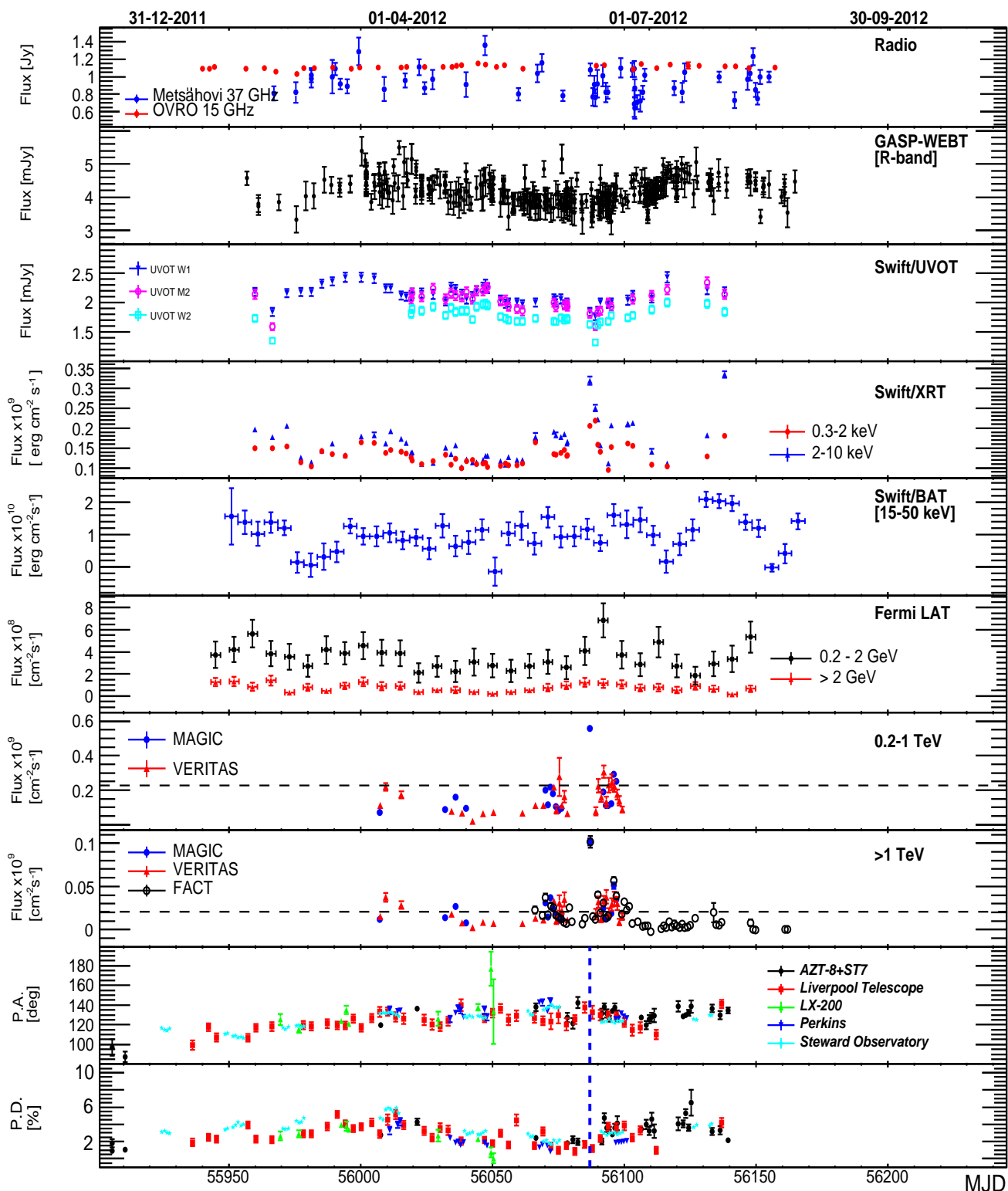
Fig. 1. Multiwavelength light curve for Mrk 501 during the 2012 campaign. The bottom two panels report the electric vector polarization angle (P.A.) and polarization degree (P.D.). The correspondence between the instruments and the measured quantities is given in the legends. The horizontal dashed line in the VHE light curves represents 1 CU as reported in Aleksić et al. (2016), and the blue vertical dotted lines in the panels with the polarization light curves depict the day of the large VHE flare (MJD 56087).
