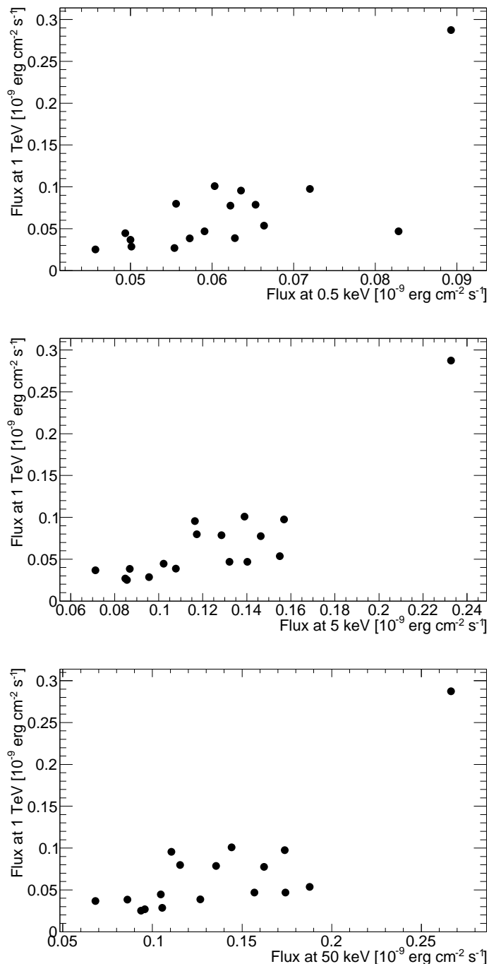
Fig. 8. Flux-flux plots derived from the one-zone SSC model used to fit 17 broadband SEDs (see Section 6). The SSC model flux at 1 TeV is compared to the SSC model flux at 0.5 keV (top), 5 keV (middle) and 50 keV (bottom). The data point with the highest X-ray and VHE activity corresponds to the one-zone SSC model for the June 9 flare (MJD 56087).
