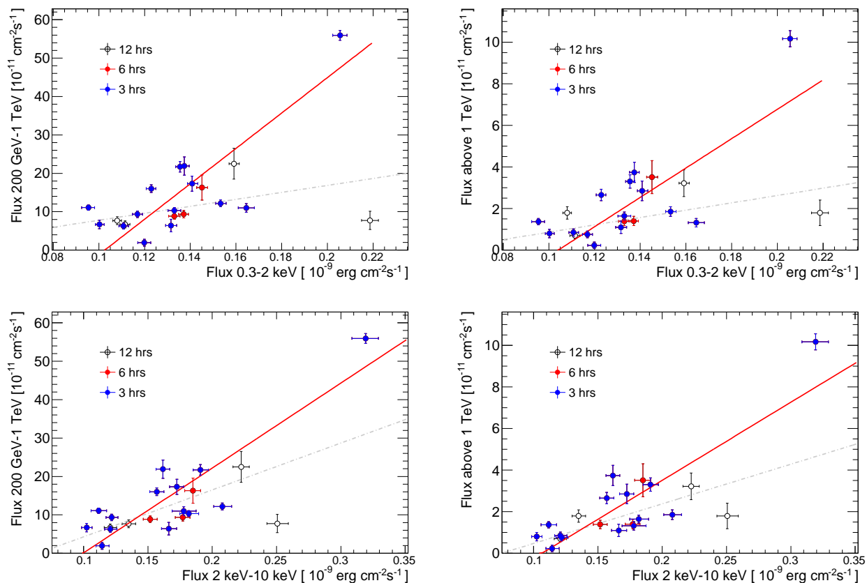
Fig. 3. VHE flux as a function of the Swift /XRT flux for the energy ranges shown. Open circles represent data that were taken within 12 hours of each other, red circles within 6 hours and blue circles within 3 hours. In each case, linear fits to the closed circle points (6 hours or less) are depicted with a red line (when considering the June 9 flare) and with a dotted-dashed grey line (when excluding the June 9 flare).
