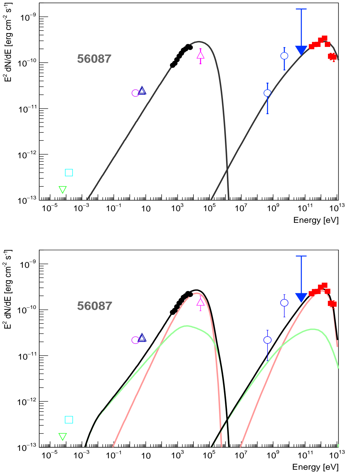
Fig. 7. Broadband SED for MJD 56087 (VHE flare from 2012 June 9), fitted with a one-zone SSC model (top) and a two-zone SSC model (bottom). See Figure 5 for explanation of markers and other details. In the bottom panel, the green line depicts the emission of the first (large) zone responsible for the baseline emission, and the red line the emission from the second (smaller) zone, that is responsible for the flaring state. The fit results from the one-zone SSC model fit are reported in Table 2, while those from the two-zone SSC model fit are reported in Table 3.
