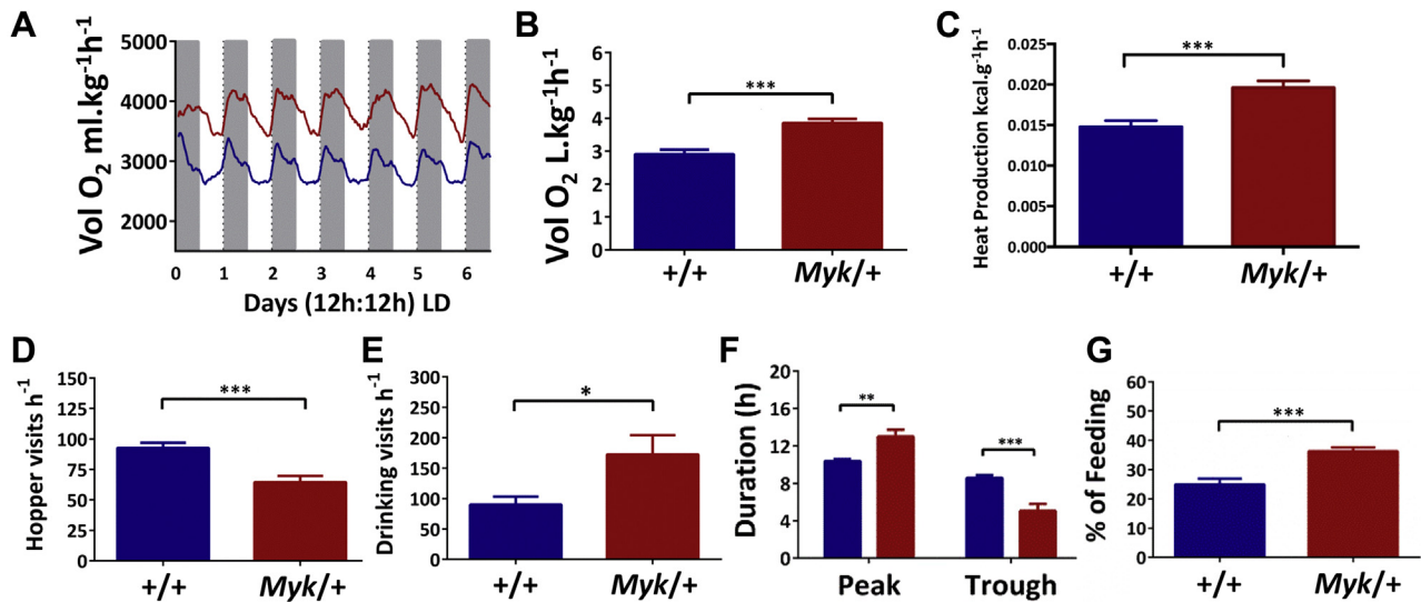
Figure 2. Altered metabolic rhythms in Myk/+ mice. (A) Smoothed traces of wild-type (+/+) mice (blue; n = 10 ) and Myk/+ mice (red; n = 12 ) maximal oxygen consumption (Vol O 2 ) over 6.5 days. Gray-shaded columns delineate lights off (dark). (B) Mean Vol O 2 consumption is elevated in Myk/+ animals (+/+ : 2.91 \pm 0.14 L/kg/hour, Myk/+ : 3.86 \pm 0.13 L/kg/hour; p < .0001 ). (C) Mean hourly heat production is elevated in the Myk/+ mice (+/+ : 0.0148 \pm 0.0007 kcal/g/hour, Myk/+ : 0.196 \pm 0.0008 kcal/g/hour; p = .0003 ). (D) Altered ingestive behaviors in Myk/+ animals. Mean hourly food hopper visits were reduced by the Myshkin mutation (+/+ : 92.6 \pm 4.3 visits, Myk/+ : 64.6 \pm 5.1 visits; p = .0005 ). (E) Mean hourly visits to drinking spout were increased by the Myshkin mutation (+/+ : 90.0 \pm 13.2 visits/hour, Myk/+ : 172.6 \pm 31.7 visits/hour; p = .03 ). (F) Altered duration of daily peak (+/+ : 10.37 \pm 0.23 hours, Myk/+ : 13 \pm 0.75 hours; p = .003 ) and nadir (+/+ : 8.59 \pm 0.30 hours, Myk/+ : 5.05 \pm 0.75 hours; p = .0004 ) in Vol O 2 activity. (G) The Myshkin mutation increases percentage of daily feeding occurring during the lights-on phase (+/+ : 25.0 \pm 1.9\% , Myk/+ : 36.3 \pm 1.3\% ; p < .0001 ). Data in panels (C–G) are plotted as mean \pm SEM. * p < .05 , ** p < .01 , *** p < .001 . LD, light/dark.
